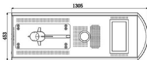
60W Model diagram
